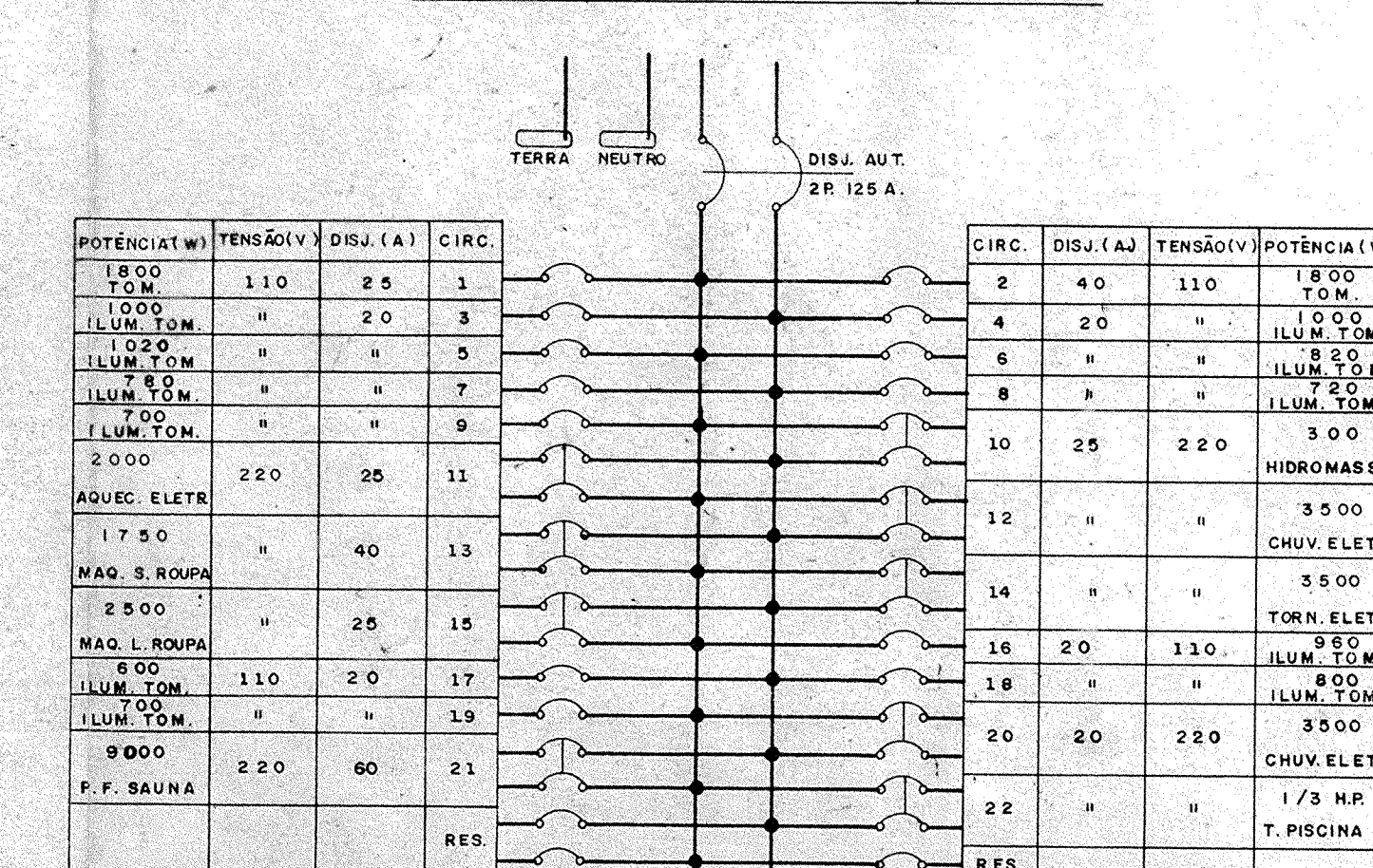
DIAGRAMA BIFILAR DO Q.L. 331, T32 DUPLEX
