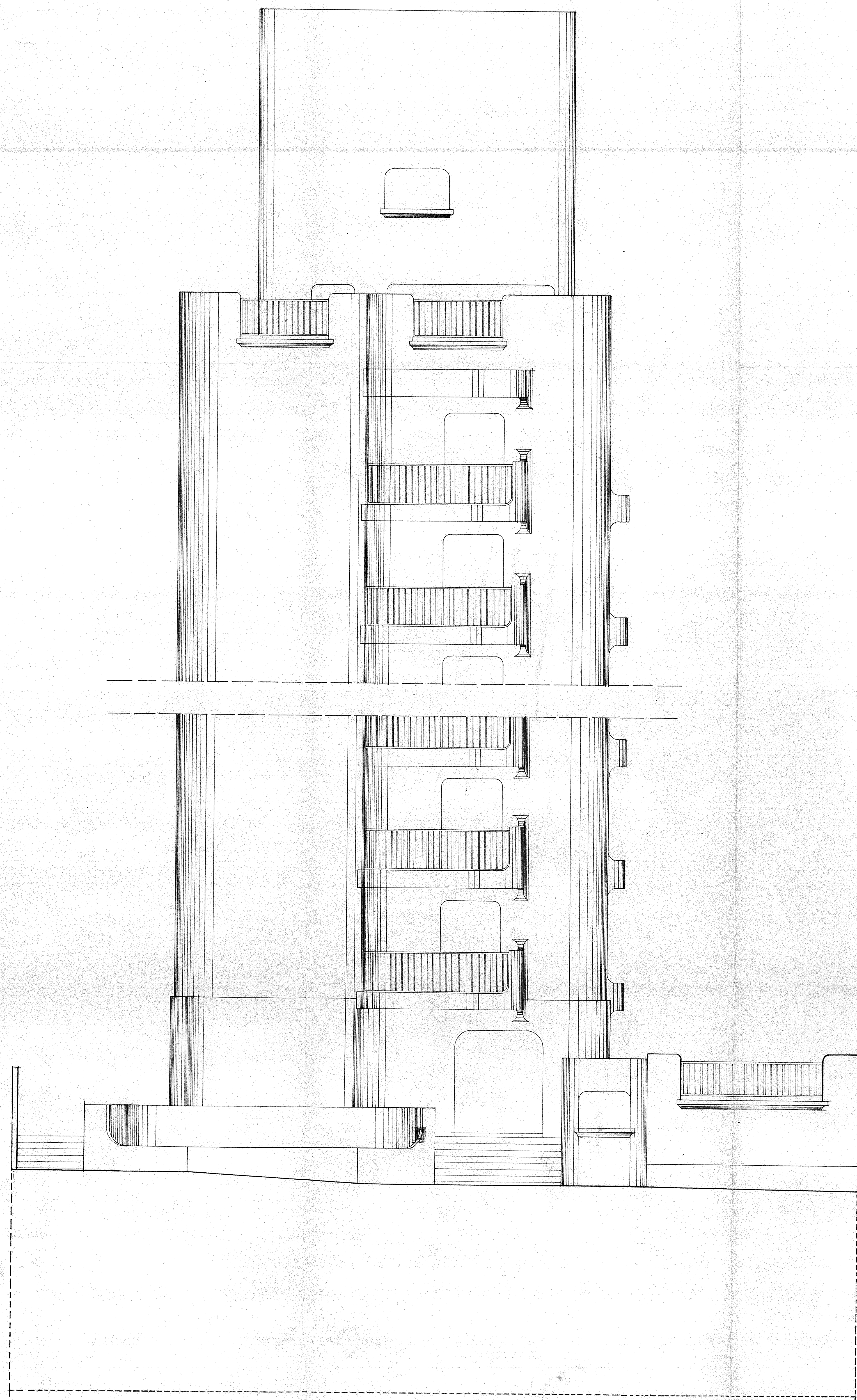
FACHADA PRINCIPAL
